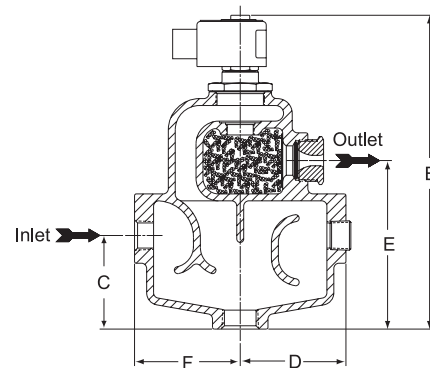
Figure 63-2. VSA humidifiers
