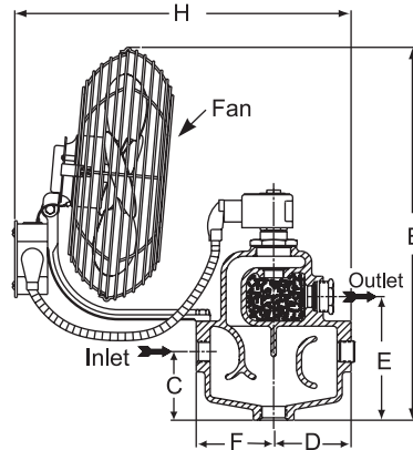
Figure 63-1. FSA humidifiers
