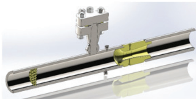
Model APTWWR – PTC-6 welded nozzle in a welded meter run with inspection port
