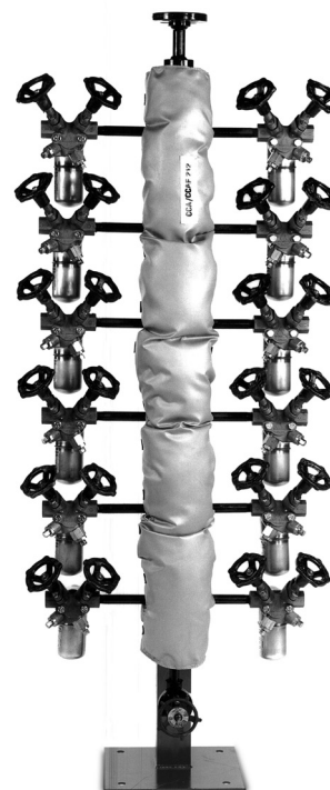
CCAF 212 Condensate Collection Assembly
