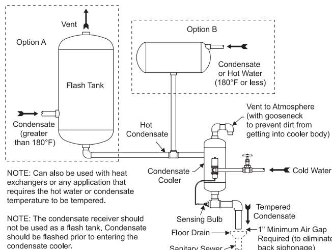
Typical Installation
