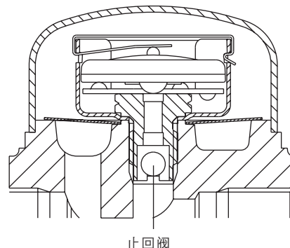
止回阀 SBP30LCV SBP30HCV
